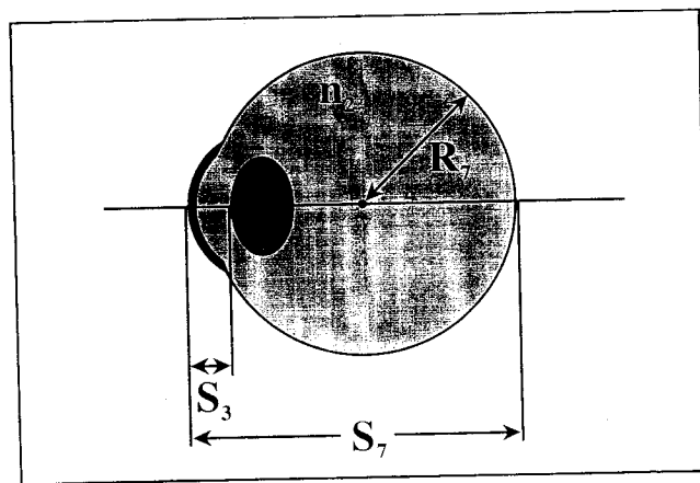
Fig. 1 The eye model presented by Gullstrand [6]; the parameters S_3 and S_7 for positions, R_7 for radius, and n_2 and n_4 for indices of refraction exemplify the notation
