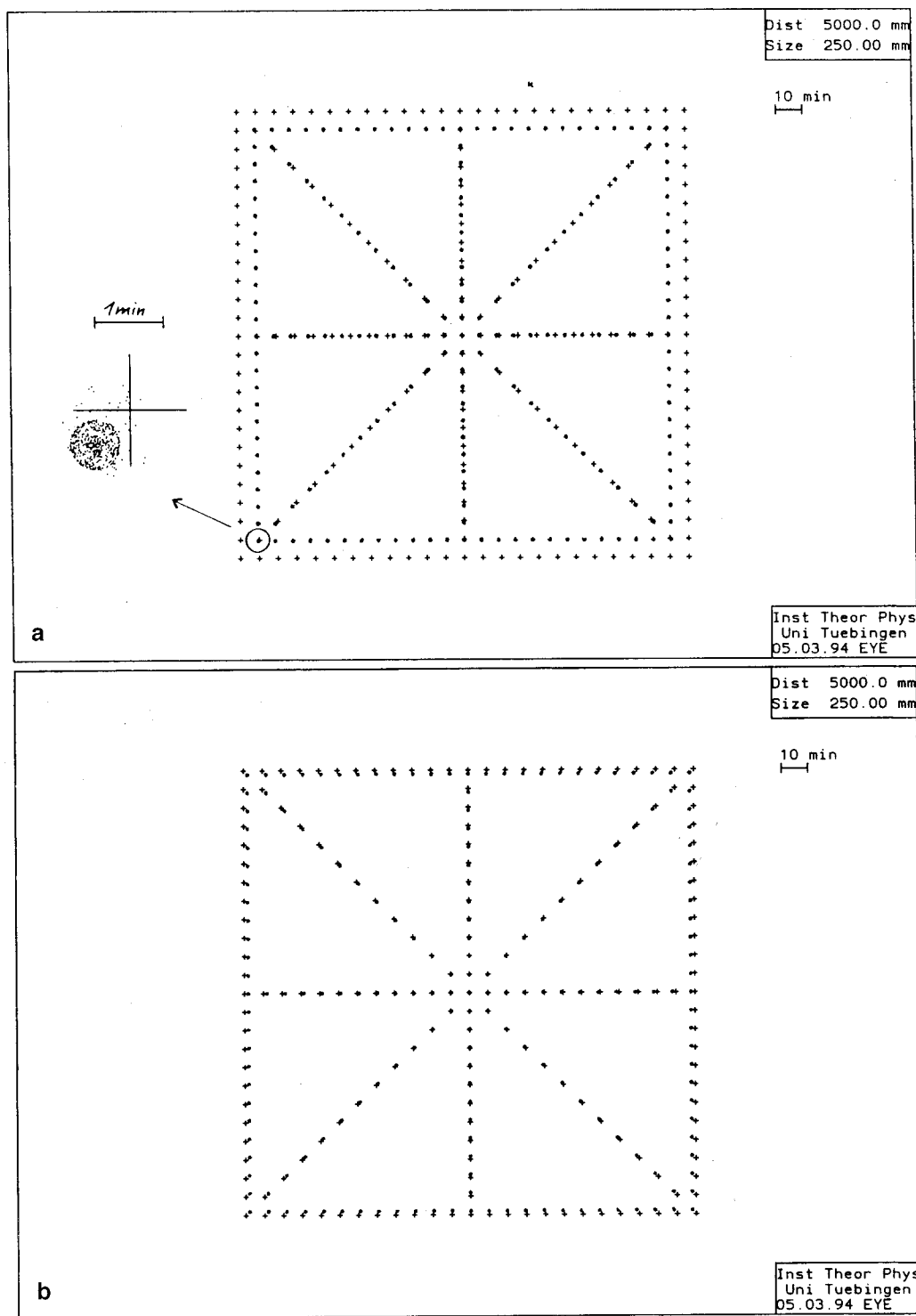
Fig. 4a, b Object and image calculated by the ray tracer. The object is a pattern of point sources (marked by crosses). The image consists of spots formed by rays intersecting the screen. a Myopic eye corrected by eye-glass of -5.0 D. b Same eye corrected by contact lens of -4.5 D
